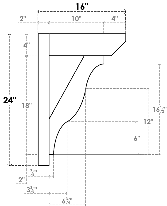
SIDE PROFILE
