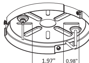
Ceiling Bracket Width of the screw slot
