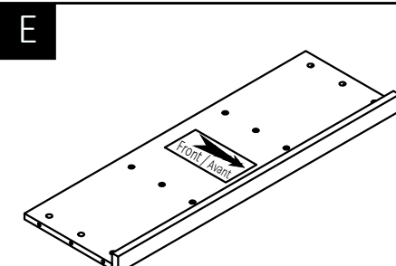
MIDDLE DIVIDER (L&R Same) QTY 2
