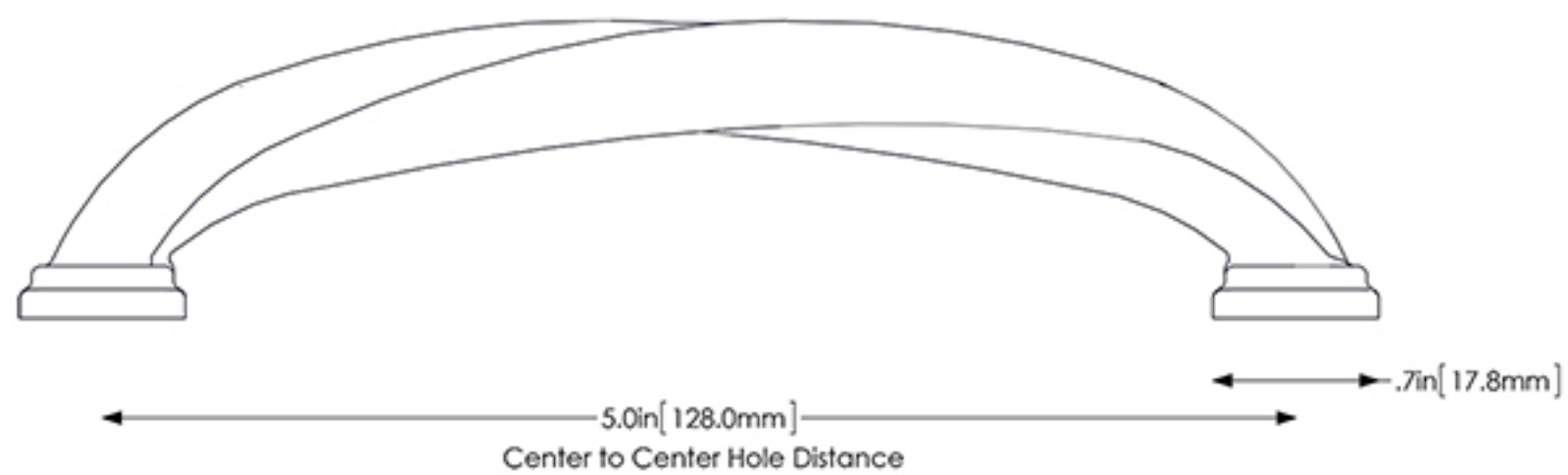
Side View
