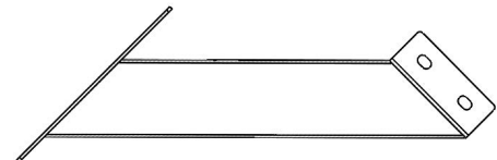
F3 | SHORT ANGLE BRACE - A4M01275 (2) | 1 1/8"x4"x14" (30x101x355)
