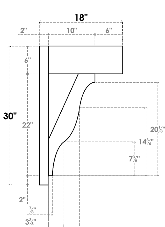
SIDE PROFILE
