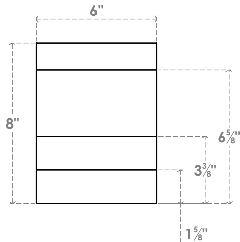
FRONT PROFILE
