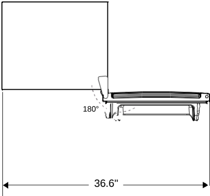
TOP OF REFRIGERATOR WITH DOOR OPEN 180°
