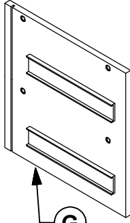
G Right Side Panel x 1
