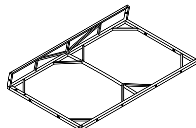
Seat right frame (1 pc)
