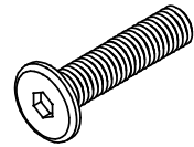
Bolt M6 x 40 mm 16 pcs + extra 2 pcs
