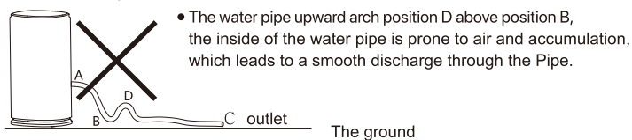
Picture 2: Example of error connection
