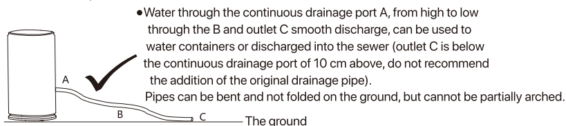
Picture 3: Example of a correct connection
