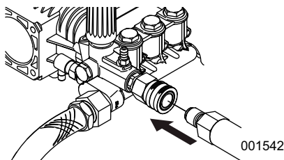
Figure 2-13. Connect High-Pressure Hose to Triplex Pump
