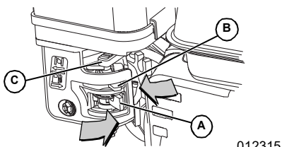
Figure 3-2. Fuel Valve and Choke
