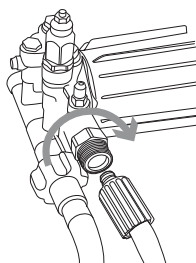
Figure 2-14. Connect High-Pressure Hose to Axial Pump (Hand Tight)
