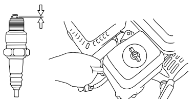
Figure 4-10. Spark Plug
