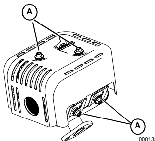
Figure 4-11. Heat Shield Fasteners
