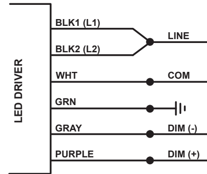
120/277 VOLT LED WIRING
