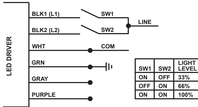
120/277 VOLT LED WIRING
