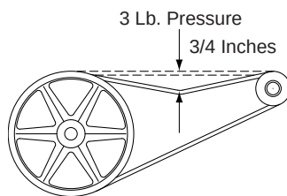
BELT TENSION
