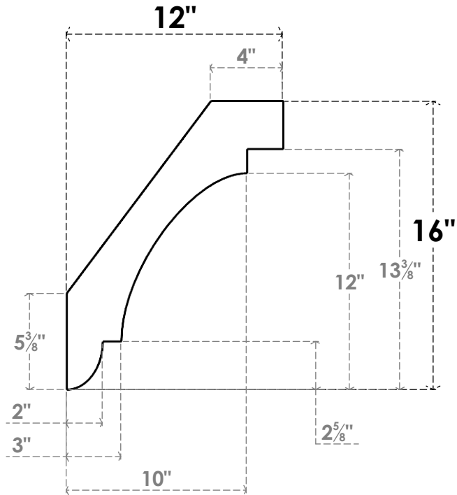
SIDE PROFILE
