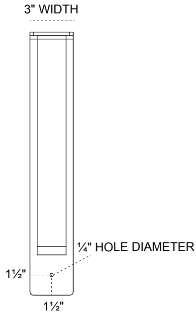
FRONT PROFILE
