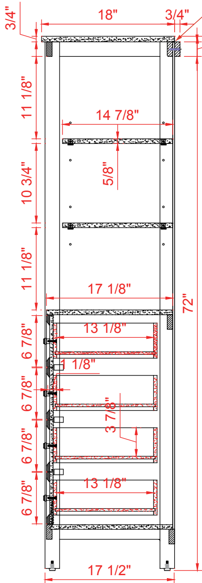
SIDE VIEW
