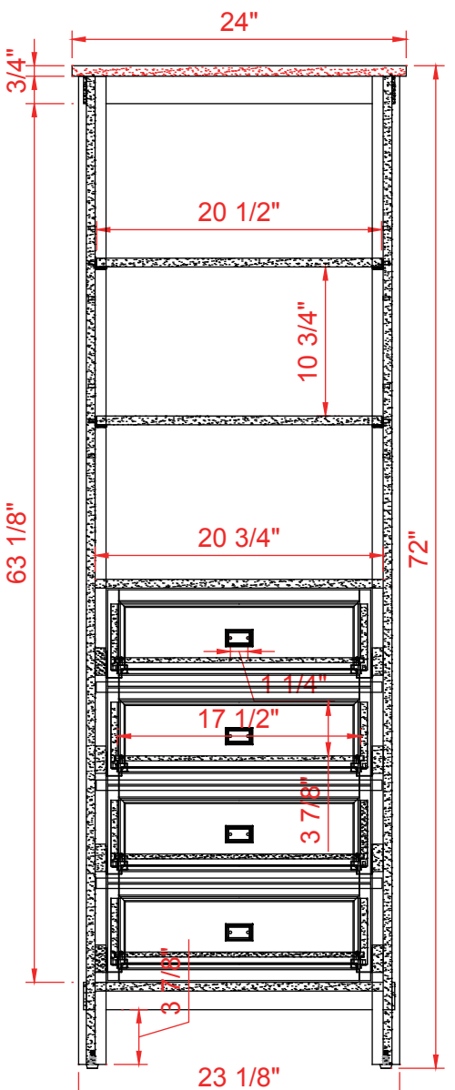
FRONT VIEW
