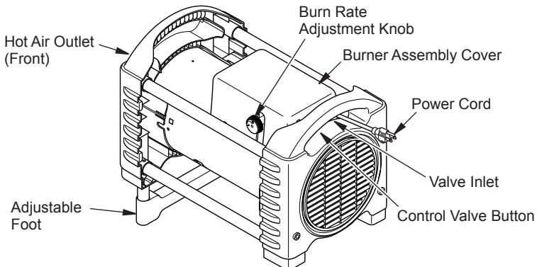
Figure 1 - 125,000 & 175,000 Btu/Hr Heater
