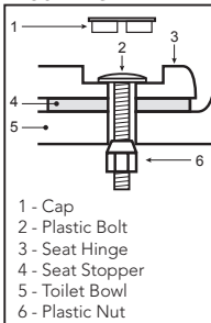
MOUNTING HARDWARE
