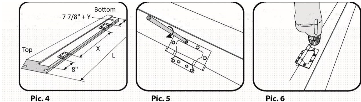
Pic. 4, 5, 6 — Marking and drilling hinge positions on the jamb
