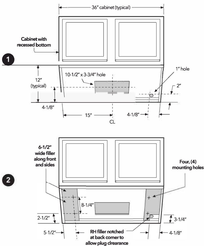
Cabinet with recessed bottom
