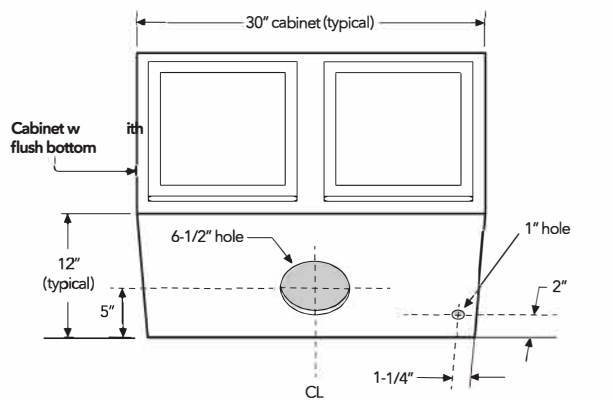
Cabinet or soffit with flush bottom
