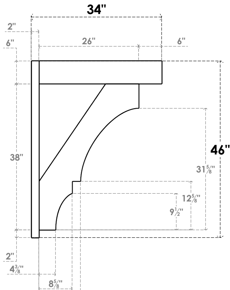
SIDE PROFILE
