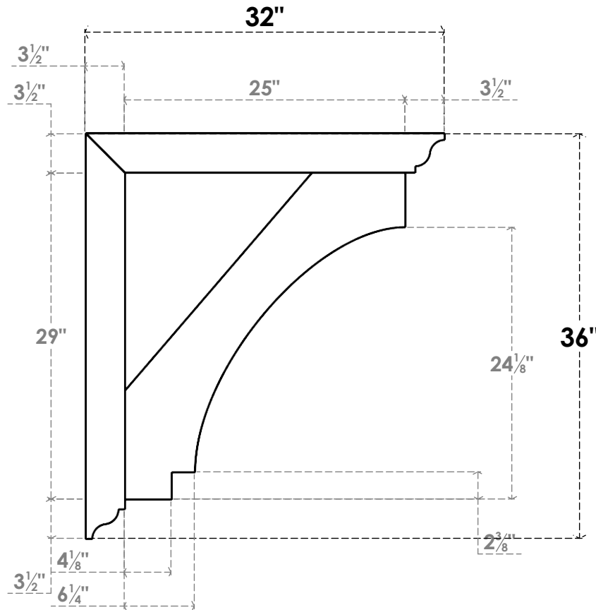
SIDE PROFILE
