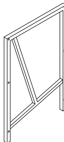
4 Side Frame Qty 2 (23.03x14.96x0.79")
