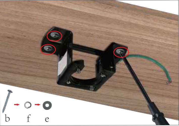
Step 1 For wooden ceiling, install the mounting plate to wooden ceiling with two wood screws.
