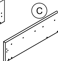
SIDE PANEL 1 T932370 X 2
