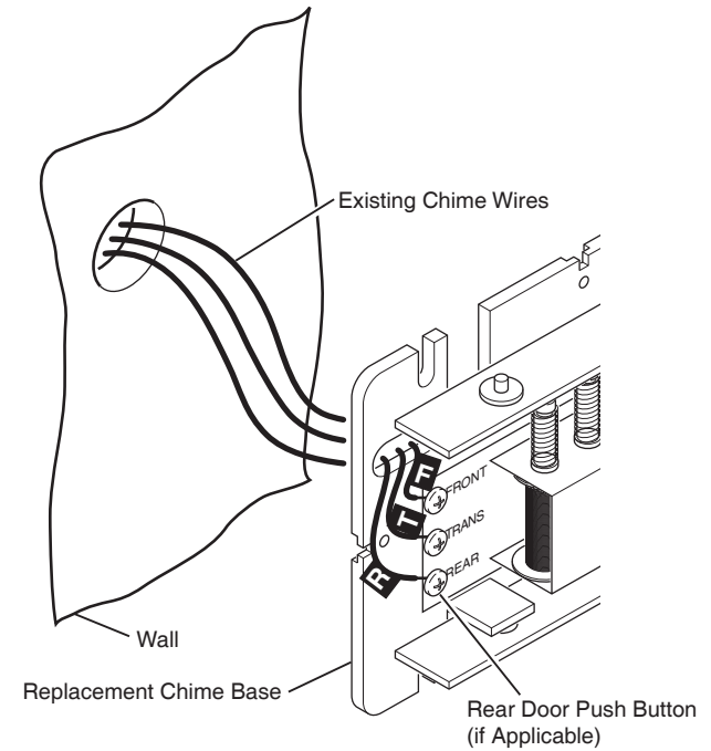
Figure 2 - Mechanical Chime Wiring
