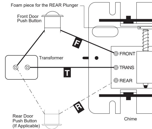
Figure 3 - Chime System Wiring Diagram
