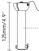
3.Downrod
