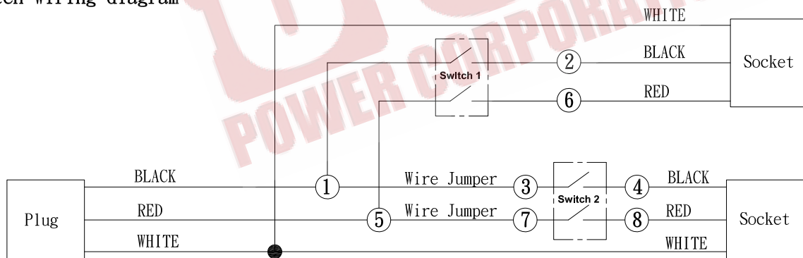
Switch Wiring diagram
