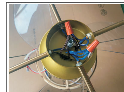
Step 5. Connect the power cable
