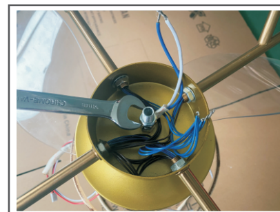
Step 4. Install fixing screws and tighten them with tools
