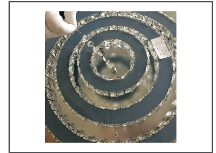
Step 5. Install one end of the crystal chain hook on the chassis of the fan lamp main engine.
