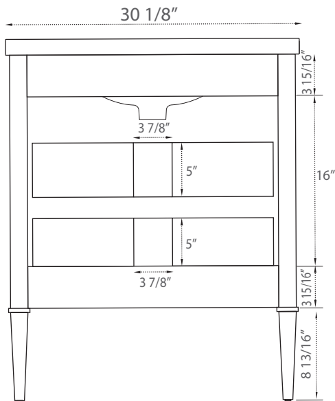
Drawer Detail
