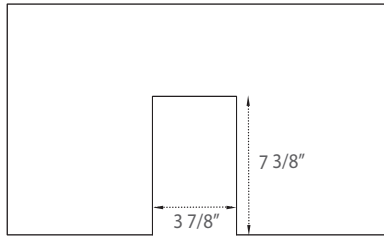
Drawer Detail
