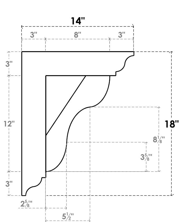
SIDE PROFILE
