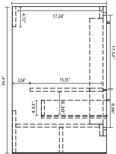
Side Elevation
