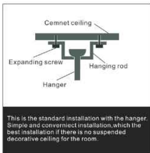
Diagram 1: Standard installation
