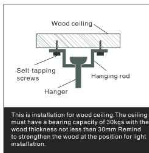
Diagram 4: Installation with wood decorative ceiling
