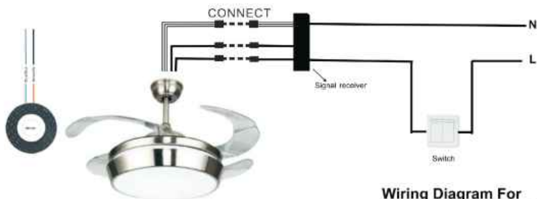
Diagram 3: Installation with suspended decorative ceiling
