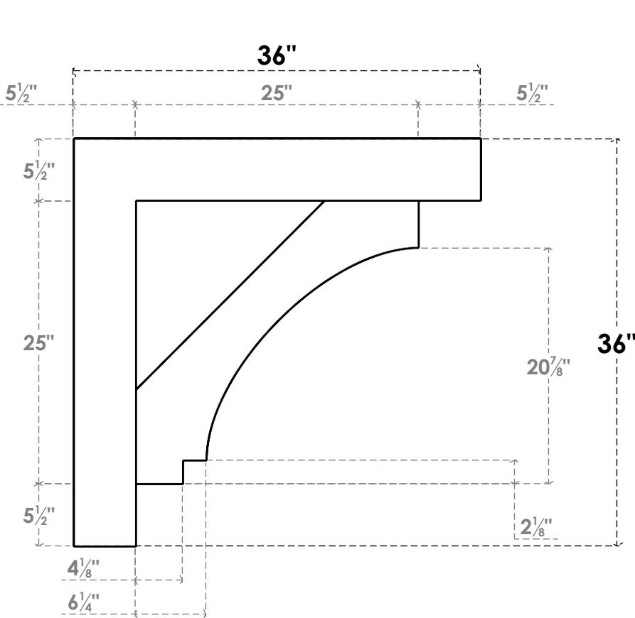
SIDE PROFILE
