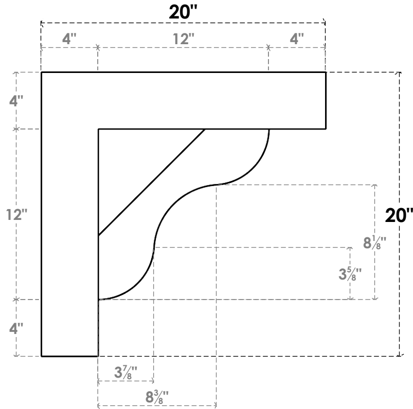
SIDE PROFILE
