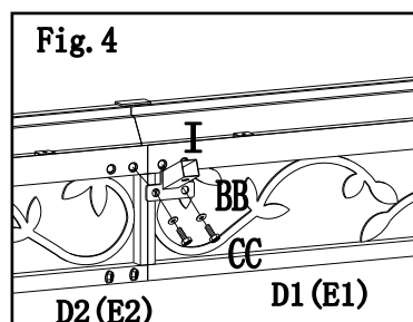
Fig.4:Attach middle beam connector(I) to frame by using bolt (CC) and washer (BB)
