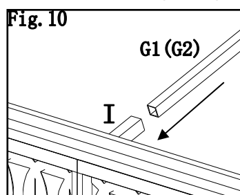
Fig.10: Insert middle beam (G1/G2) to middle beam connector (I) .
