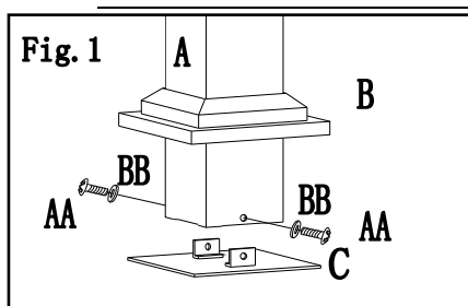
Fig.1:Put Base cover (B) through Post (A) and lift up base cover, then attach base (C) to bottom of post (A) by using bolt(AA)、washer (BB).
