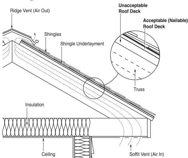
Figure 4-2: An acceptable deck applied over an unacceptable deck.
