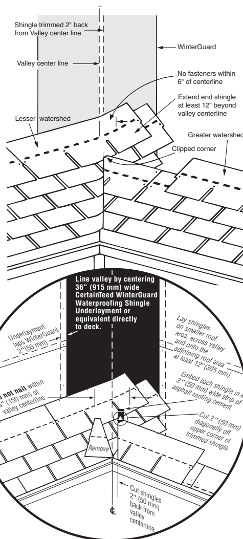
Figure 6-17: Closed-cut valley application.
