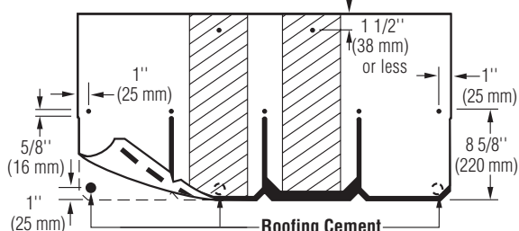
Figure 17-5: When installing Grand Manor on steep slopes, use seven nails and three spots of asphalt roofing cement.
