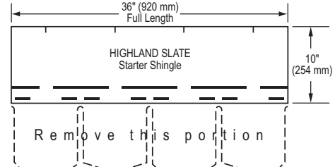
Figure 15-4: Make starter shingles by removing the lower 8" portion.
