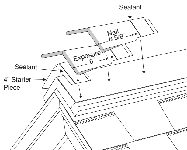
Figure 12-16: Hip and ridge application.
