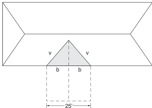
Figure 3-8: Valley Length (v), ell roof
