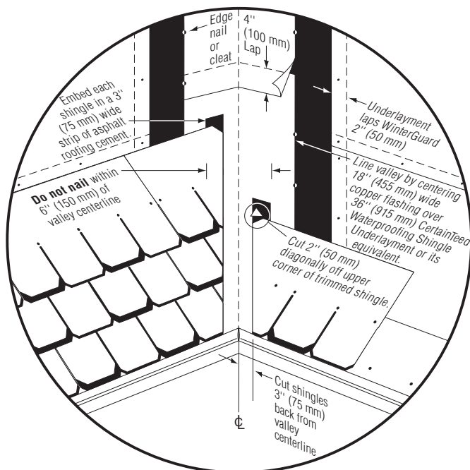
Figure 17-11 Valley installation for Grand Manor®.
