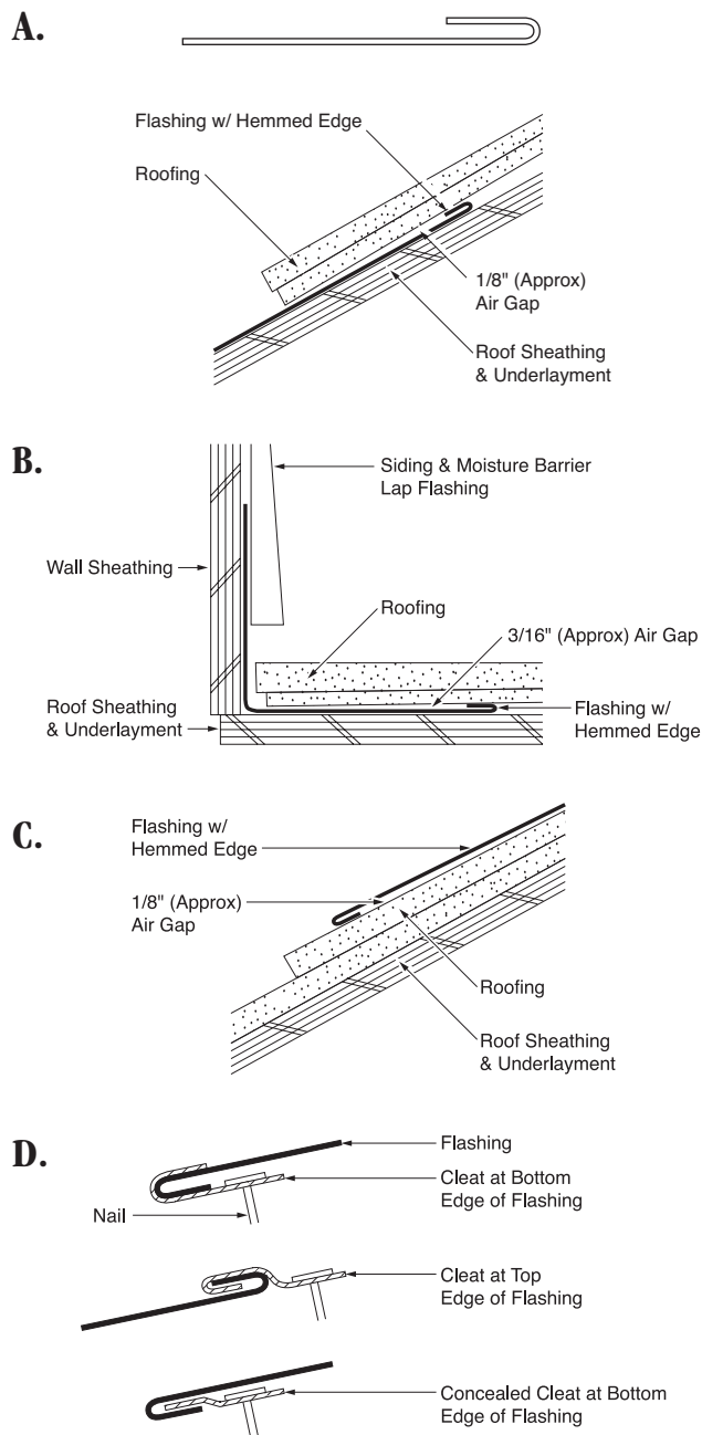
Figure 6-27: The hemmed edge is a very important detail or roof flashing.
