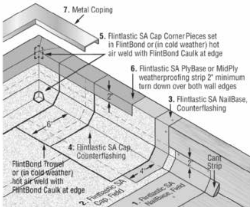
Inside Corner 2 Ply
