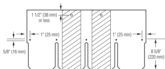
Figure 16-3: Use five nails for every full shingle.
