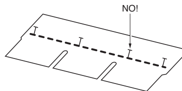
Figure 1-5: Avoid nailing into sealant strips.
