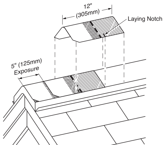
Figure 12-15: Use laying notches to center shingles on hips and ridges, and to locate the correct exposure.
