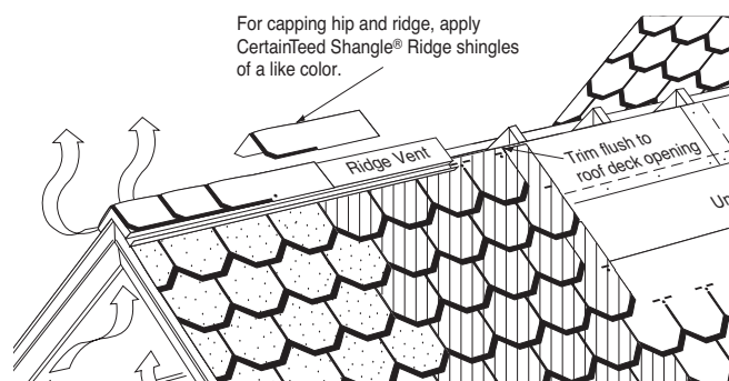
Figure 17-20: Installation of Shangle Ridge shingles on ridge vent.
