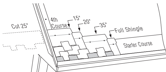
Figure 14-15: Fourth Course.
