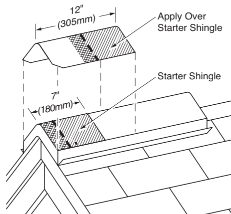
Figure 12-12: Apply a full cap shingle over the starter piece, flush with the bottom and side edges of the starter.
