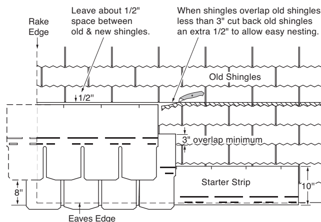
Figure 16-18: “Cutback/Nesting Method”
