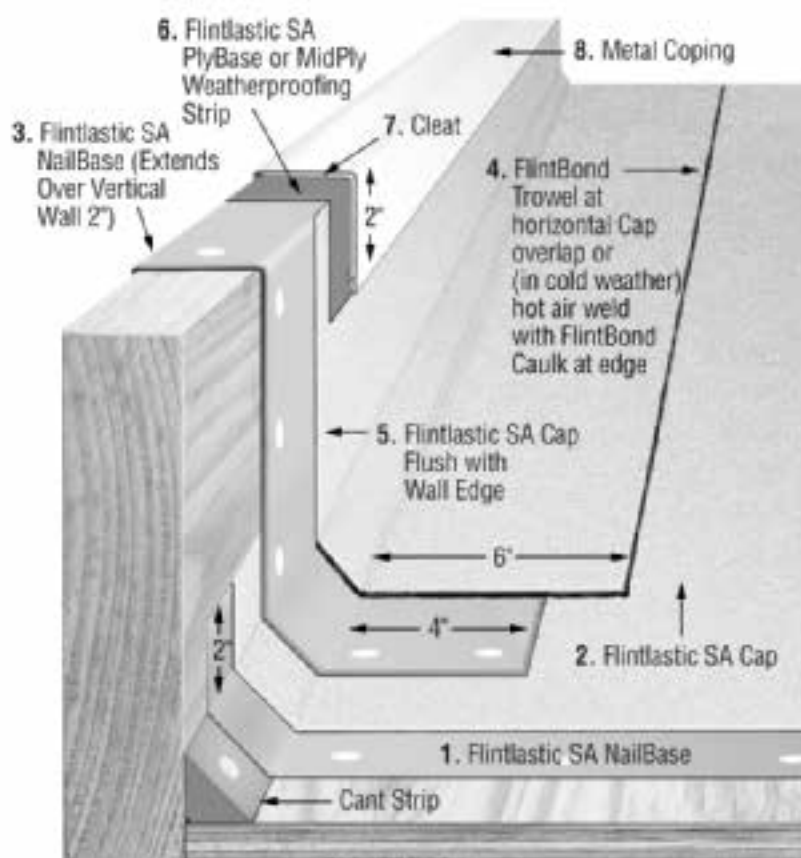
Parapet Wall 2 Ply
