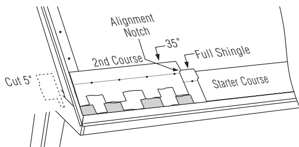
Figure 14-13: Second Course.
