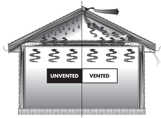
Figure 7-2: Unvented: Moisture rising up through the house condenses in the attic, causing damage to studs, insulation, and other materials.
