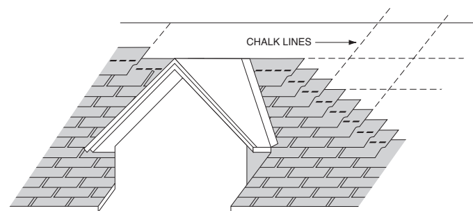
Figure 9-11: Ensure shingles on the main roof continue the same alignment pattern on both sides of the dormer as shown.
