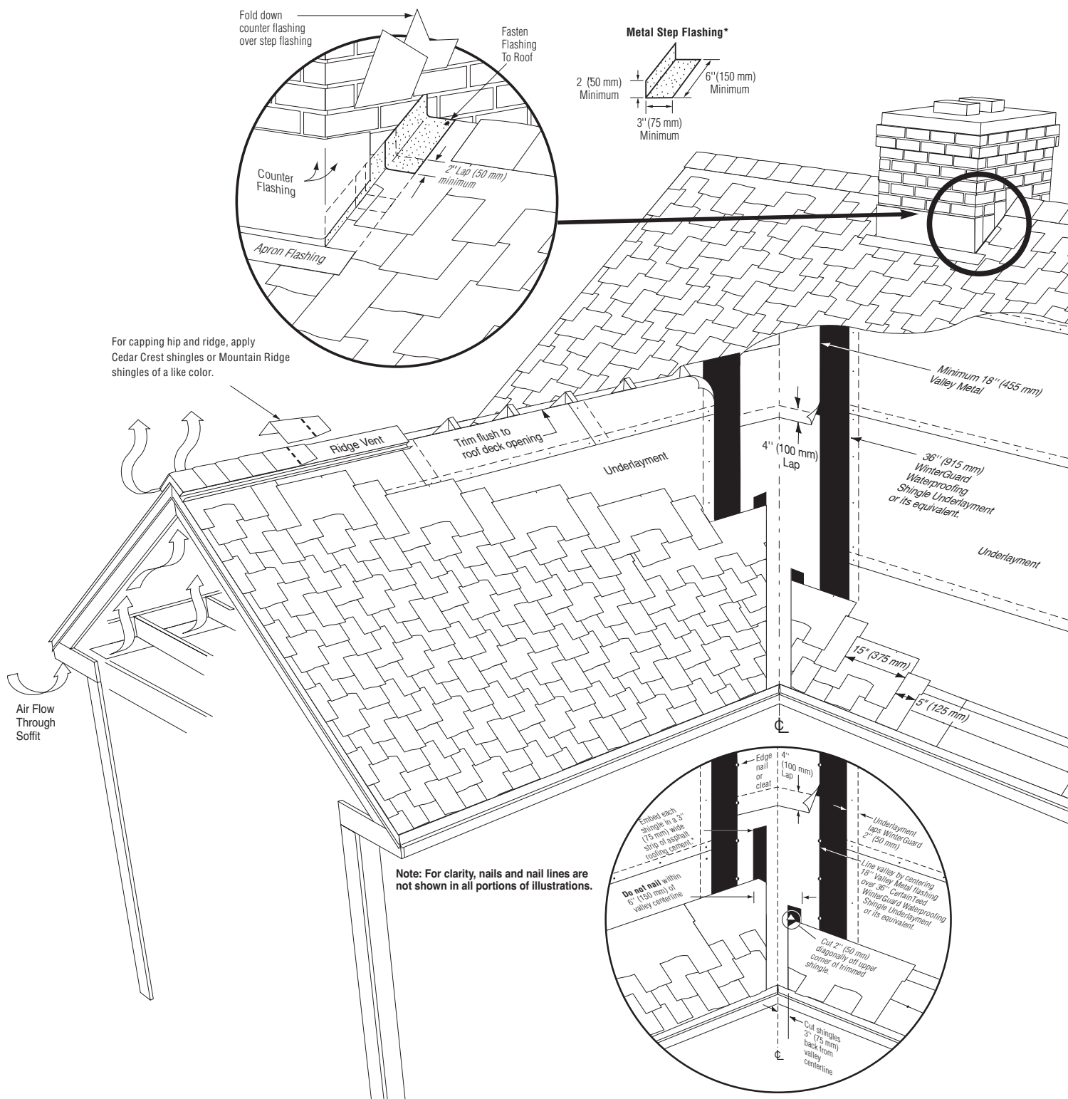
Figure 14-16: Highlight of open valley and chimney flashing details.
