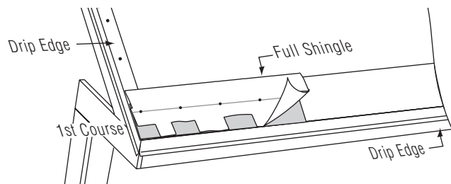
Figure 14-12: First Course.
