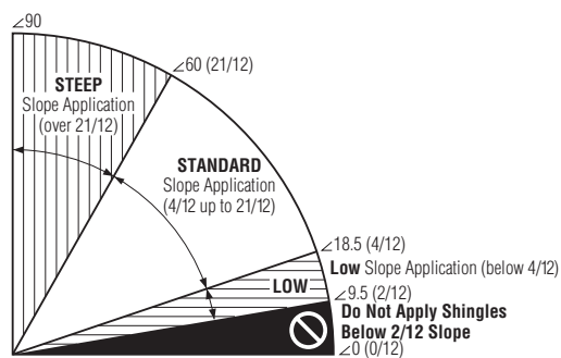
Figure 14-4: Slope definitions
