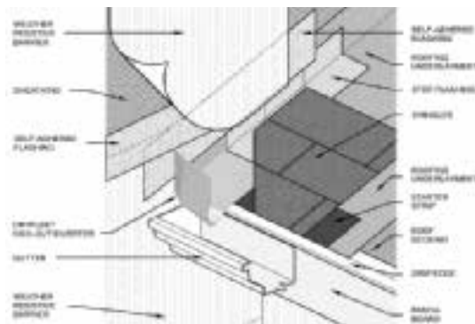
Kick-out Diverter
