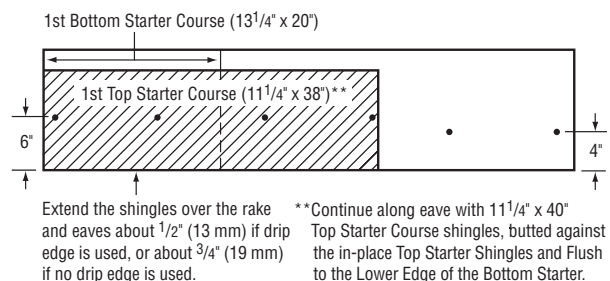
Figure 14-11: Use two (2) overlapping layers of CertainTeed's "Presidential Starter."
