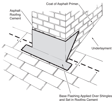
Figure 6-9: Chimney base flashing application.
