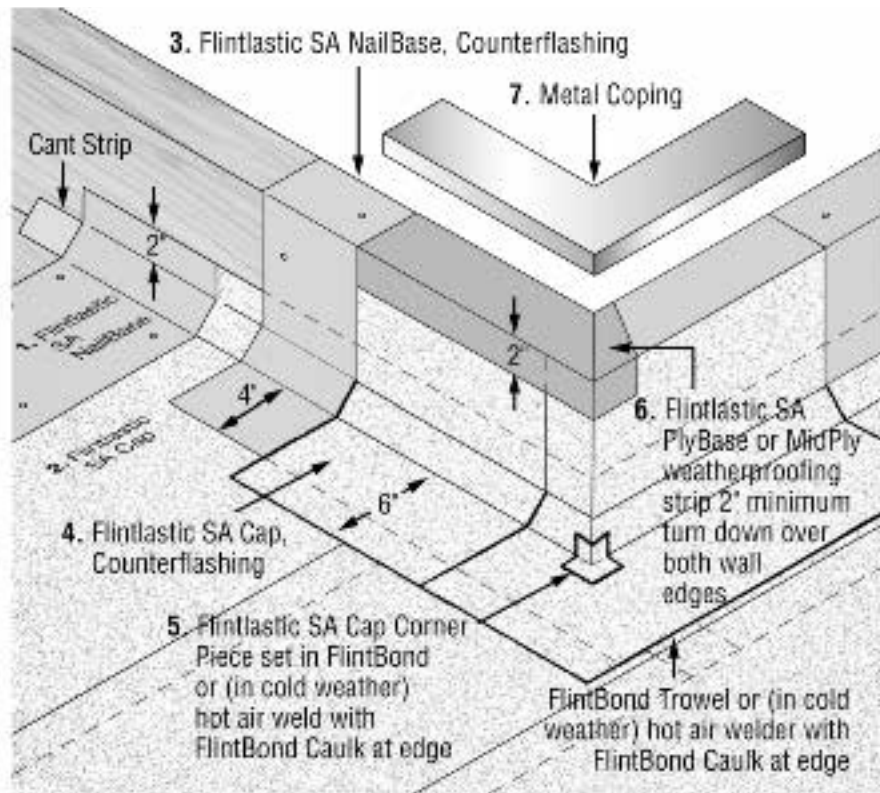
Outside Corner 2 Ply
