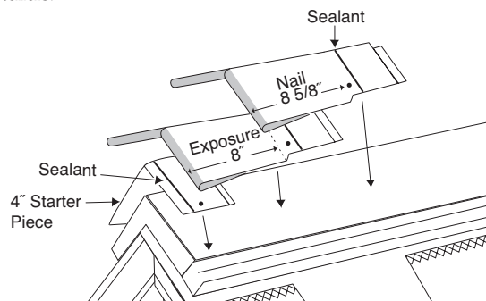
Figure 14-17: Mountain Ridge Hip and ridge application.
