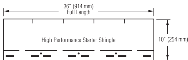
Figure 16-6: High-performance starter shingle.
