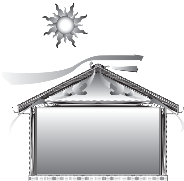
Figure 7-7: Thermal Flow (effect whereby cooler air falls, warmer air rises) and Natural Flow (effect due to wind) come together to ventilate an attic.
