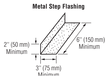
Figure 14-23: Metal step flashing.
