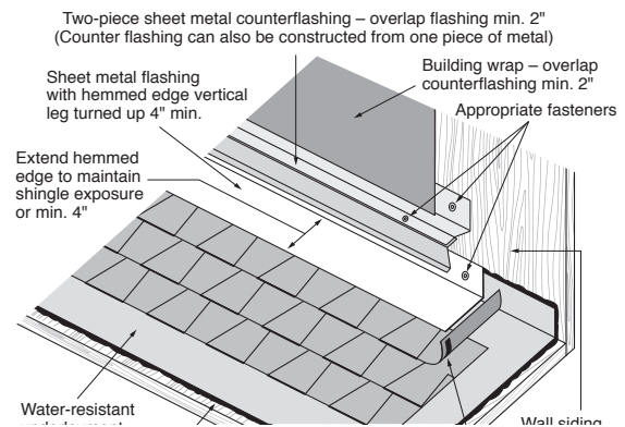
Figure 6-4a: An alternate front wall flashing method.
