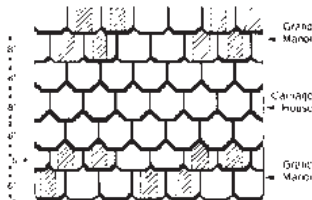
Figure 17-21: Blending Carriage House® with Grand Manor®.
