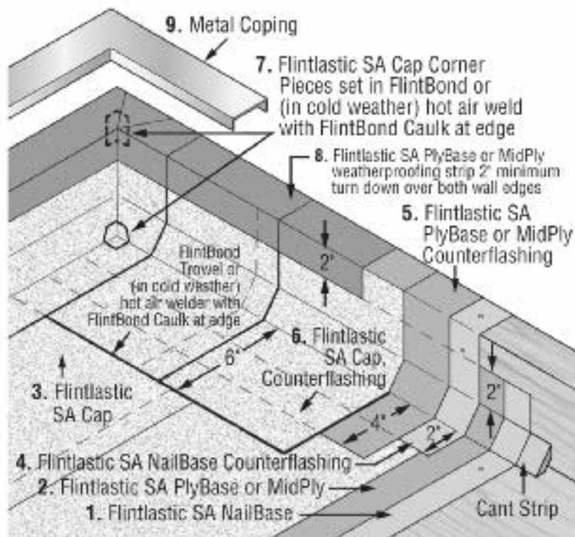
Inside Corner 3 Ply
