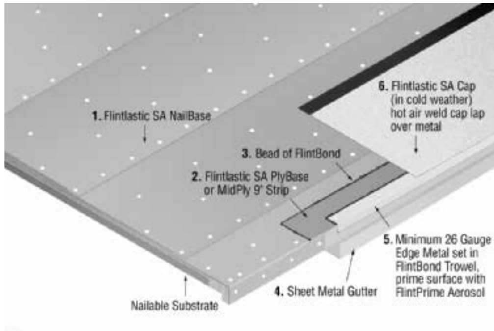
Rain Gutter Edge Detail 2 Ply
