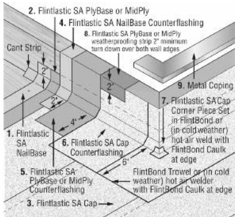
Outside Corner 3 Ply
