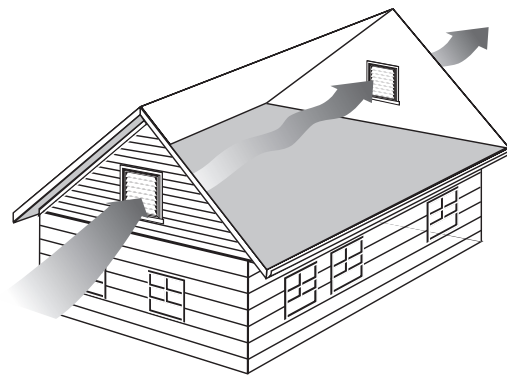
Figure 7-18: With wind blowing perpendicular to the ridge, the louvers act as both intake and exhaust vents.
