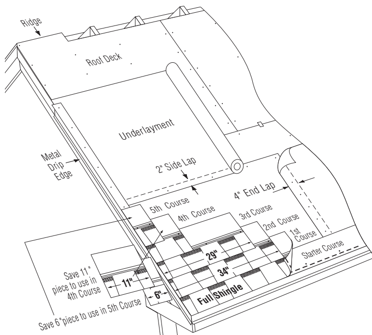
Figure 12-6: Applying the first 5 courses of Landmark TL.
