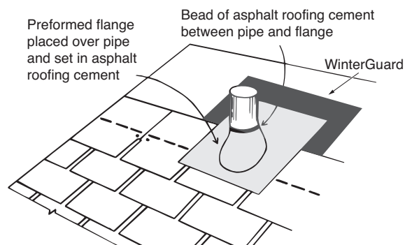
Figure 6-6: Placement of flange over vent pipe.
