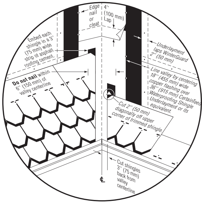
Figure 17-12: Valley installation for Carriage House®.
