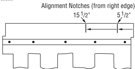
Figure 14-8: Use the alignment notches to ensure shingles are applied at a 5" and 15" diagonal offset.
