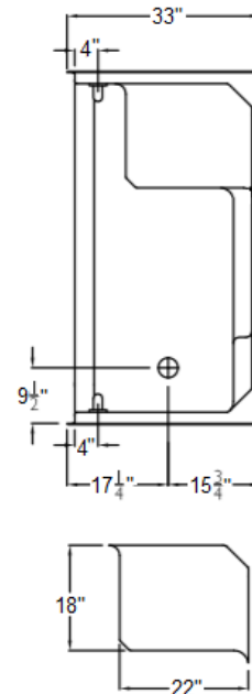
SEAT SIZE
