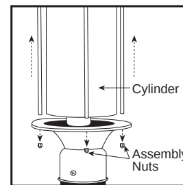
Figure 5 Cylinder Fixtures
