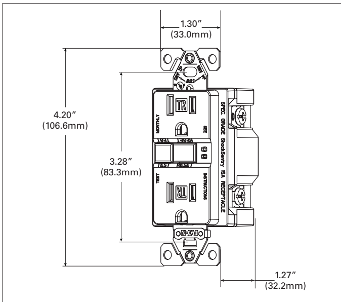
Figure 3. TRSGF15 Line art with dimensions
