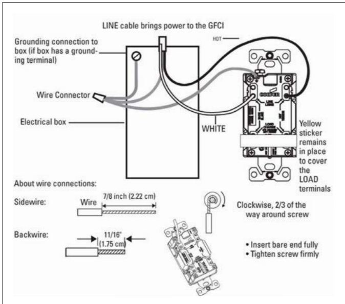
Figure 1. One cable (2 or 3 wires) entering the box
