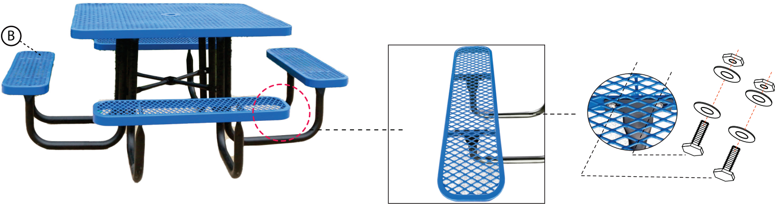
Step 3 Connect the bench to the table legs
