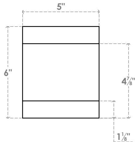
FRONT PROFILE
