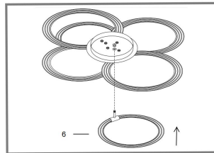
Step 7: Fix 6th ring's thread pole to the ceiling case by the nut which through the wire
