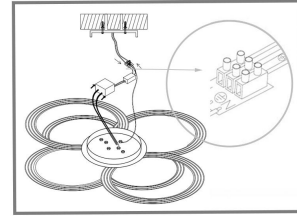
Step 9: Connect the wire through the terminal block.
