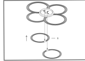
Step 6: Fix 5th ring's thread pole to the ceiling case by the nut which through the wire
