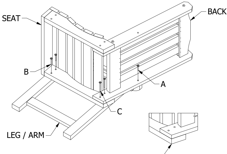
BACK ALIGNMENT
