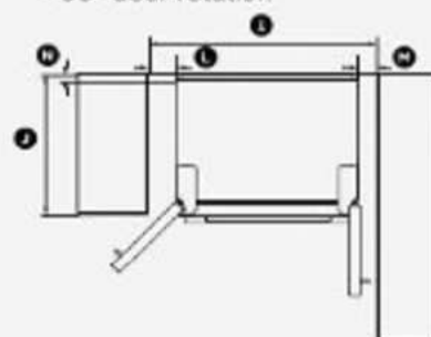
Plan View Flush with refrigerator door - 90° door rotation
