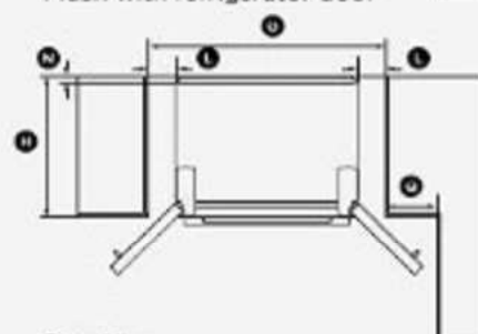
Plan View Flush with refrigerator door - 90° door rotation
