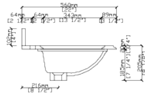
RIGHT VIEW
