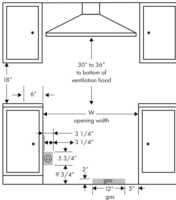
Front View
