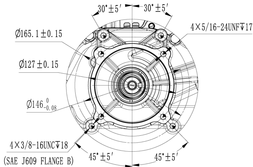
DETAIL B
