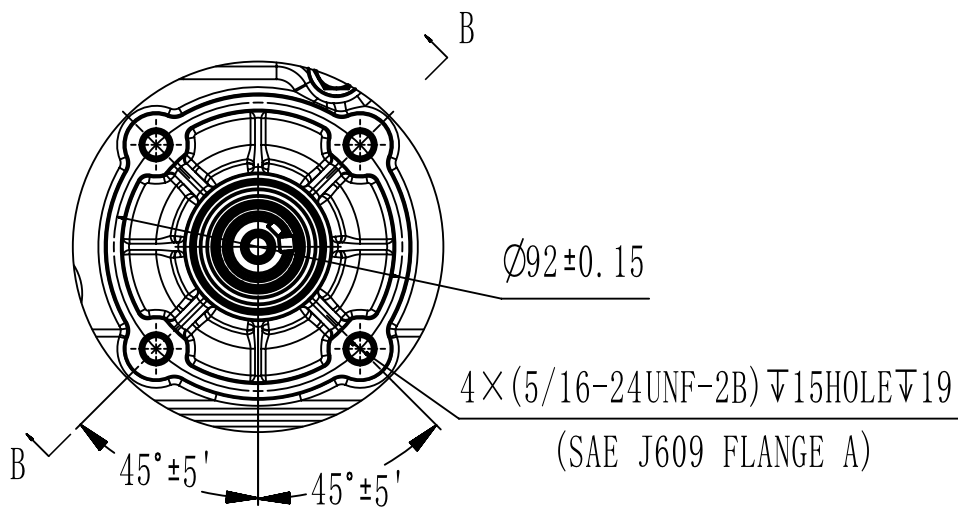
DETAIL A
